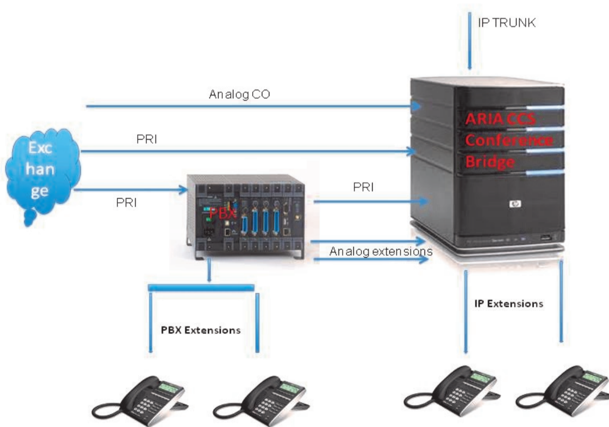
ARIA CCS- CONFERENCE BRIDGE NETWORK DIAGRAM
